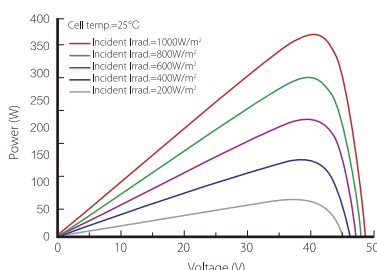
Power-Voltage Curve (LR6-72PE-360M)
