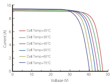
Current-Voltage Curve (LR6-72PE-360M)
