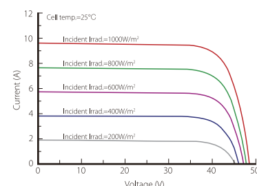
Current-Voltage Curve (LR6-72PE-360M)
